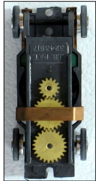
Aurora Thunderjet 500 Hollow Rivet Chassis Top View
