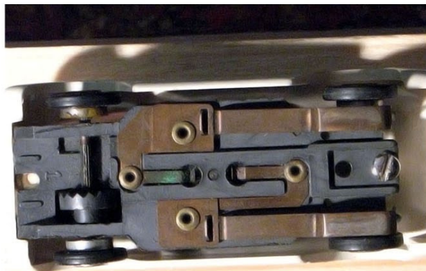
After a bit of shelf time any chassis can get like this. Oxidation and corrosion rob power from the motor
