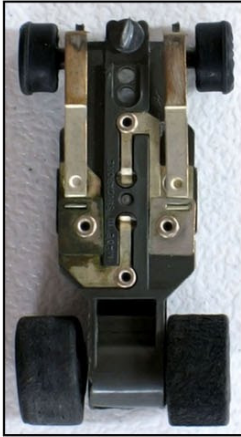
Aurora AFX Specialty Chassis Bottom View
