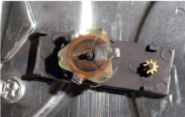
Here's the stock T-Jet armature straight from the chassis. It can use a little TLC.
