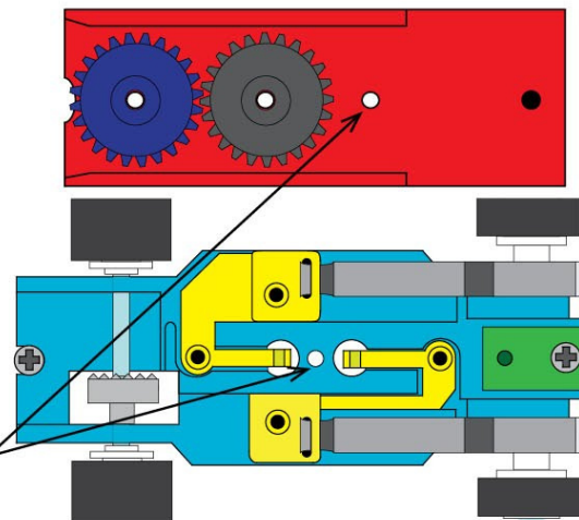
Armature Bushings
