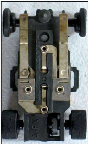
Aurora AFX 1st Generation Chassis Bottom View
