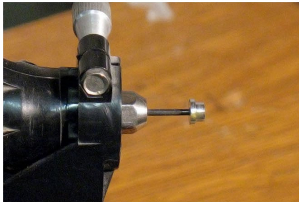
By using a straight axle and a moto-tool, you can true up any problems you find with the stock rims.
