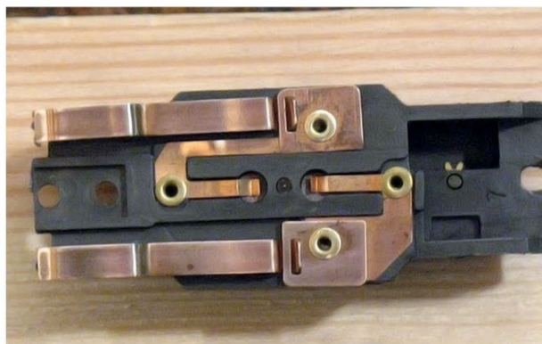
Using a mild abrasive polish, clean connections can be restored. Make sure to wipe away any residue left by the polishing compound.
