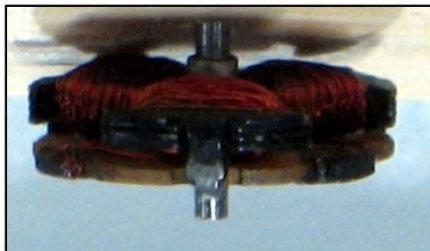
Aurora AFX Quad-Lam Armature Side View
