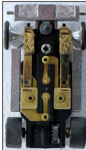
Aurora AFX Super II Chassis Bottom View
