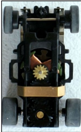
Auto World X-Traction Chassis Bottom View
