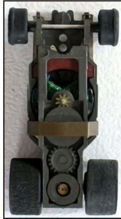
Aurora AFX Specialty Chassis Top View
