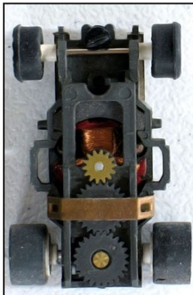
Aurora AFX Magna-Traction Chassis Top View
