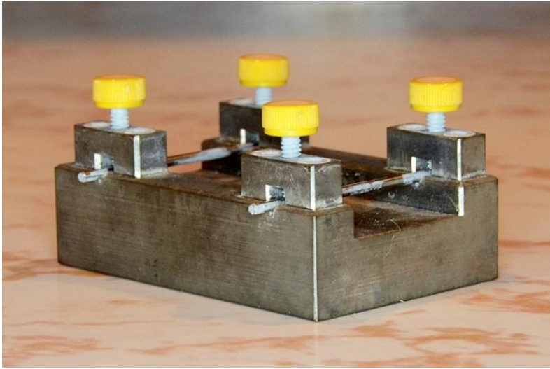
Boiling fixture
