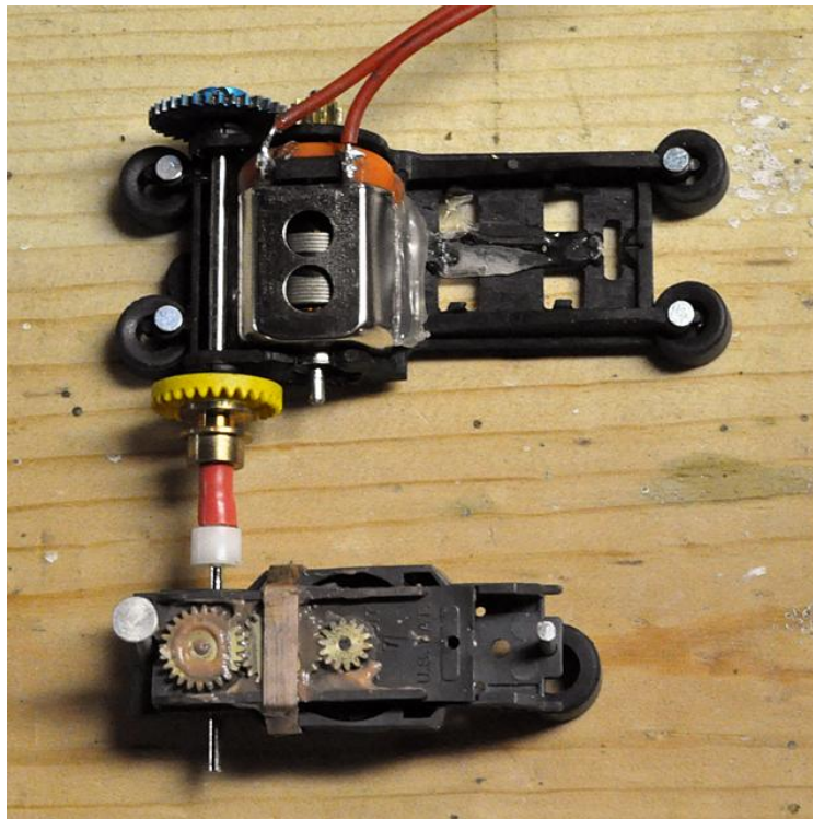
Gear lapping rig
